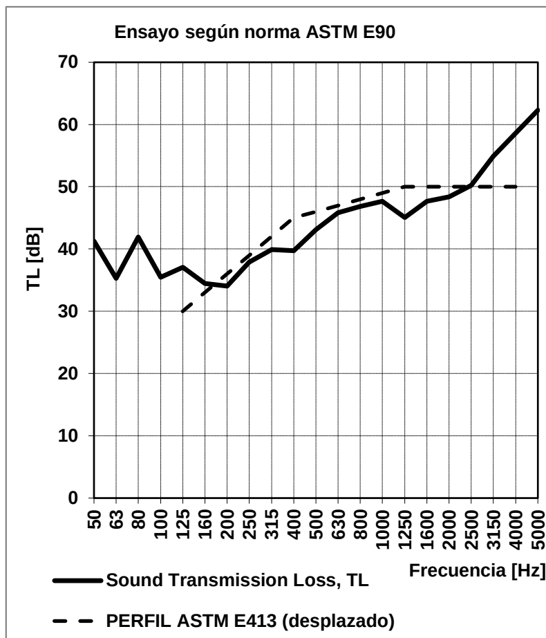
Gráfico 2: Sound Transmission Loss
